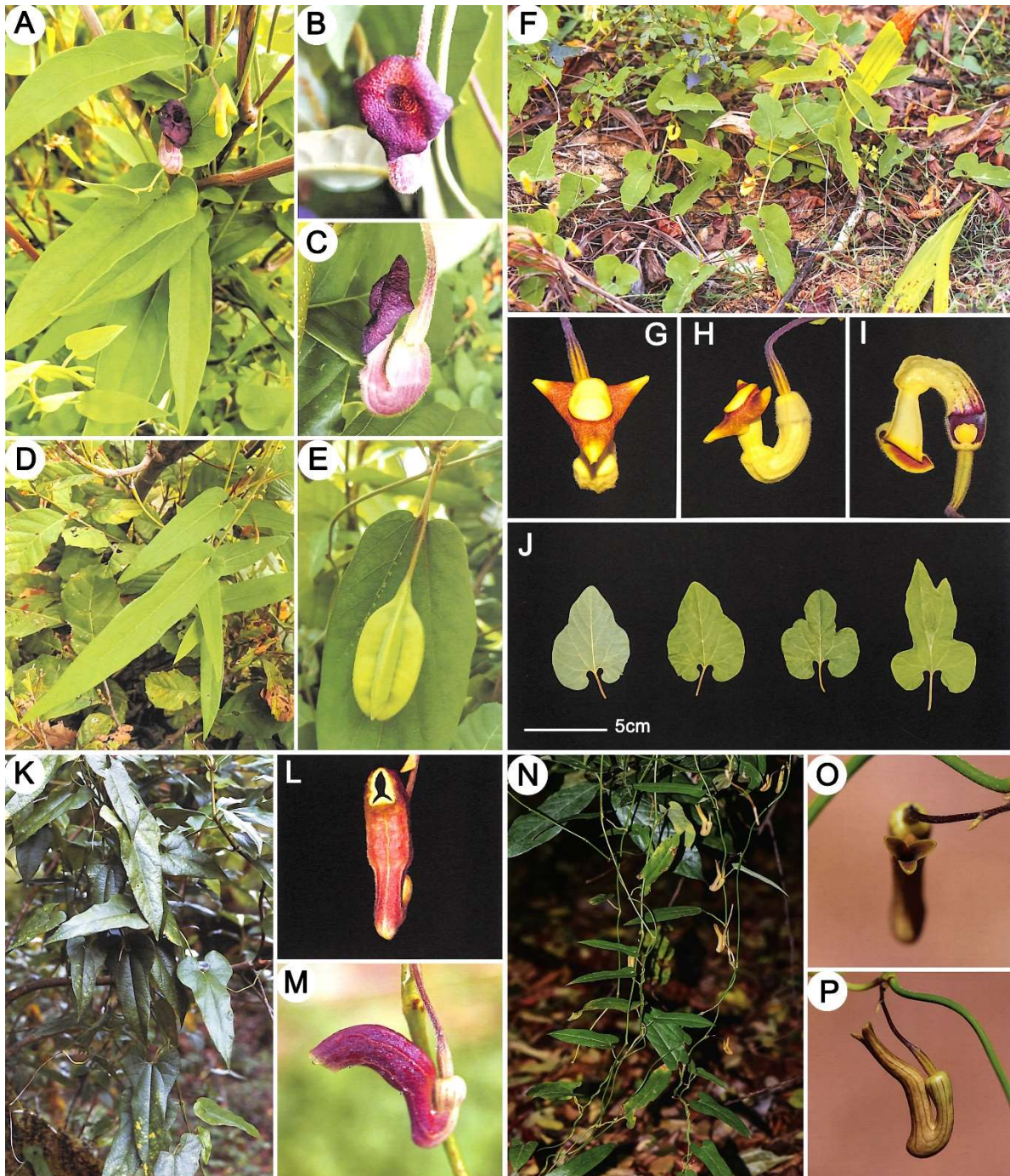
Fig. S1. A-E: Isotrema liangshanense (Z. L. Yang) X. X. Zhu, S. Liao & J. S. Ma. A: Flowering branch. B-C: Flower (front view and lateral view). D: Leaves. E: Fruit. F-J: Isotrema heterophyllum (Hemsl.) Stapf. F: Habit. G-H: Flower (front view and lateral view). I: Longitudinally dissected flower. J: Leaf blades (adaxially and abaxially view). K-M: Isotrema wardianum (J. S. Ma) X. X. Zhu, S. Liao & J. S. Ma. K: Habit. L-M: Flower (front view and lateral view). N-P: Isotrema cucurbitoides (C. F. Liang) X. X. Zhu, S. Liao & J. S. Ma. N: Habit. O-P: Flower (front view and lateral view). Note: All pictures of Fig. S1 are cited from Ma et al. 2022.
