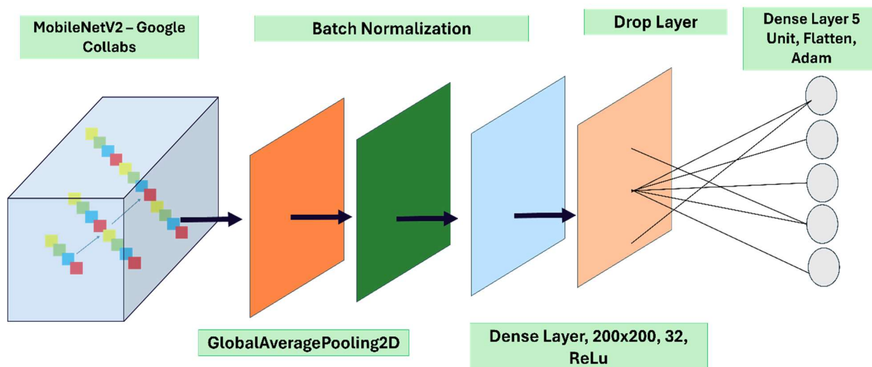
Fig. 2. MobileNetV2 architecture.
