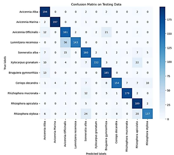
Fig. 6. Confusion matrix for large model (Left), small model (Right) at epoch 50 for training data, validation data, and testing data using real dataset
